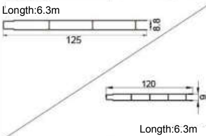
Model:YDL-8306C Thickness:0.6mm Name: gusset board Weight per meter:0.457kg/m
