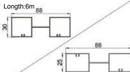
Model: YDL-19067 Thickness: 0.8mm Name: bright window Weight per meter: 0.646kg/m
